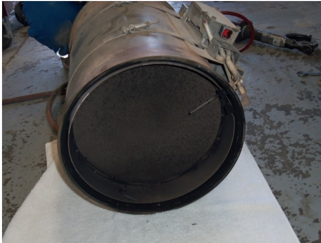
Untreated DPF from CAT powered Fracking Pump Truck
